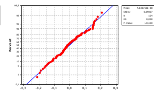
b. Residual \ln \hat{Y}_{2it}
