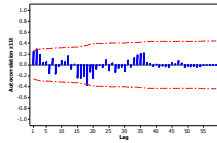
Gambar 1. Plot ACF data penjualan market sepeda motor
