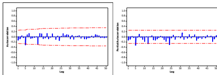
Gambar 2. ACF dan PACF plot a_t model penjualan total market
