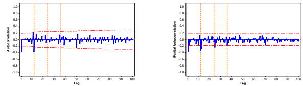
Gambar 8. Plot ACF dan PACF Differencing (1,12)
