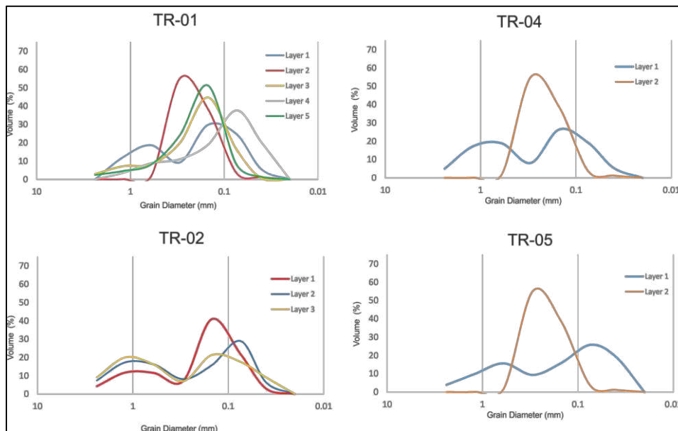
Fig 3. Seve analysis that shows percentage of grain size distribution of each layer at four location (TR-01, TR-02, TR-04, and TR-05).
