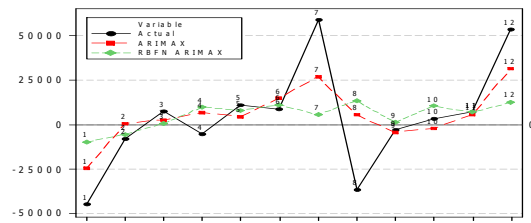
Gambar 6. ARIMAX vs RBFN ARIMAX (27-2-1)
