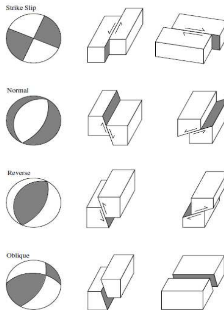
Gambar 2.2. Hubungan Focal Spheres dan Fault Geometries (Shearer, 2009)
