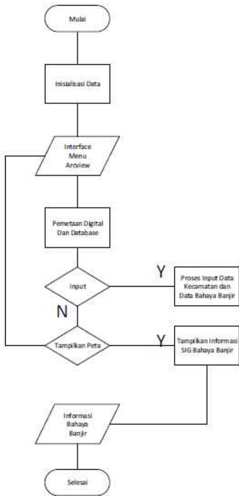
Gambar 1. Flowchart Sistem
