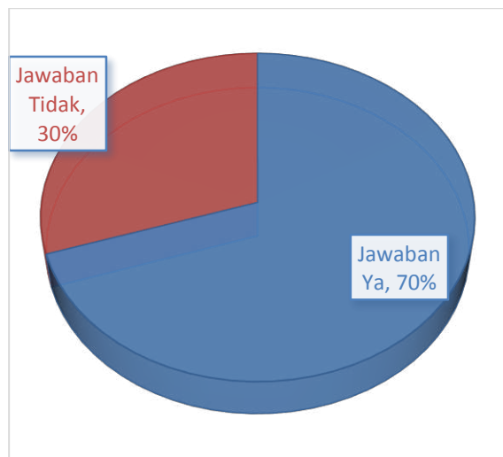
Gambar 14. Hasil Persentase
