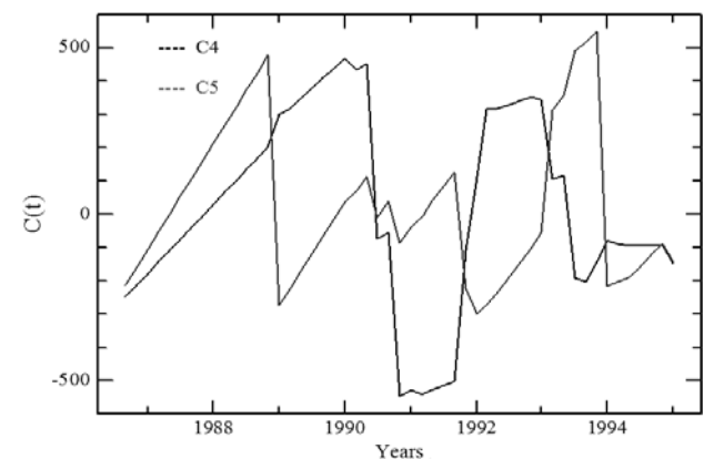
Figure 9. Fourth and Fifth Temporal Eigen-function c_4(t) and c_5(t)
