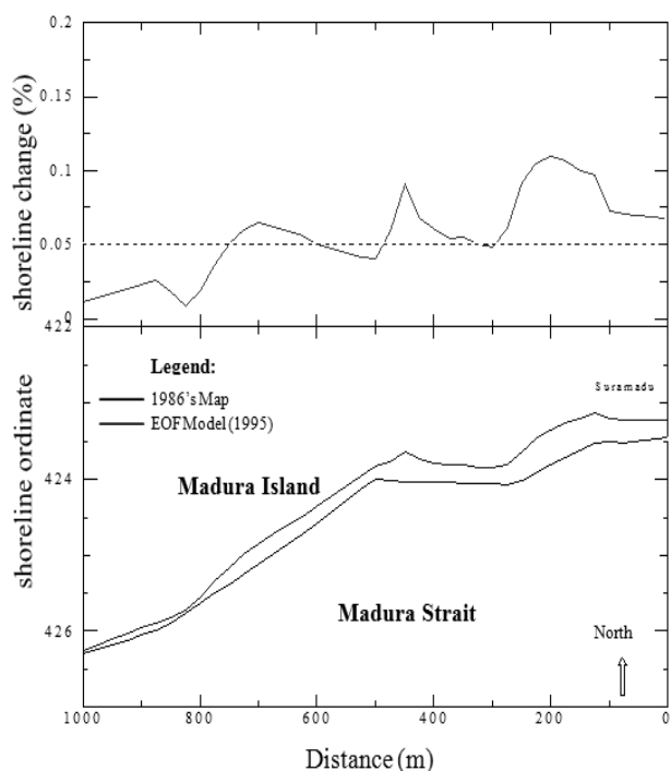
Figure 15. Shoreline Conditions: Details on Cells 1-40
