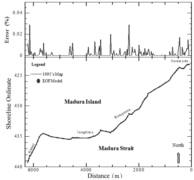
Figure 12. 1995's Shoreline by EOF Model with Maps Data
