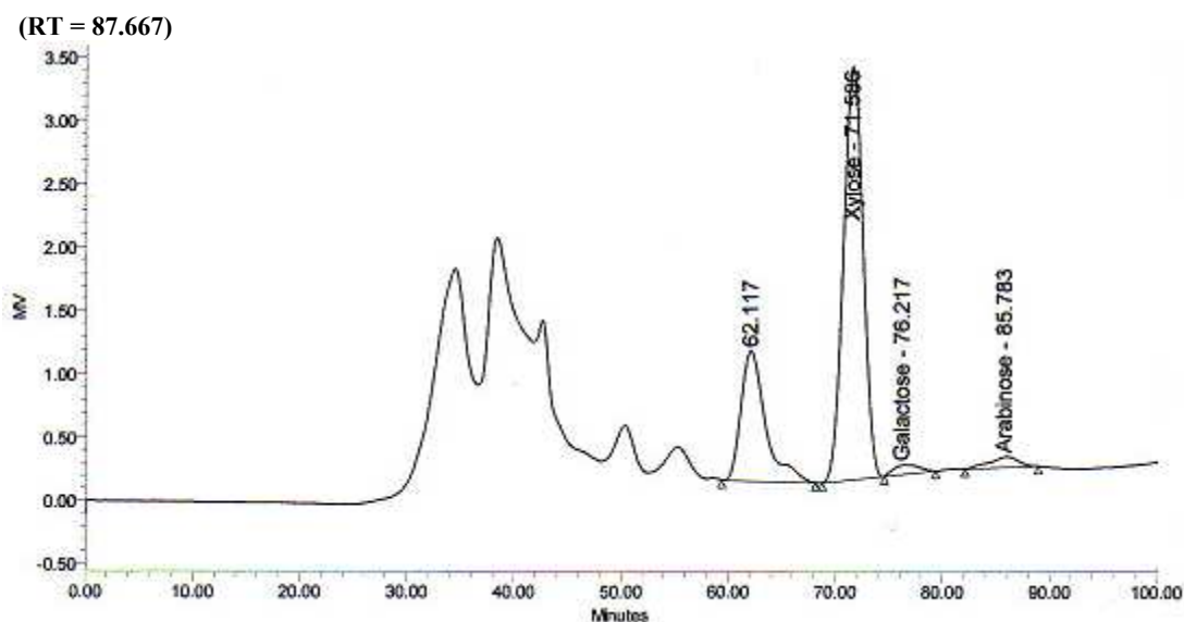
Figure 8. HPLC Chromatogram of Hydrolysis Products of Enzyme Mixture of Exo-xyl and Xyl : Xylose (RT = 71.586), Arabinose (RT = 85.783)
