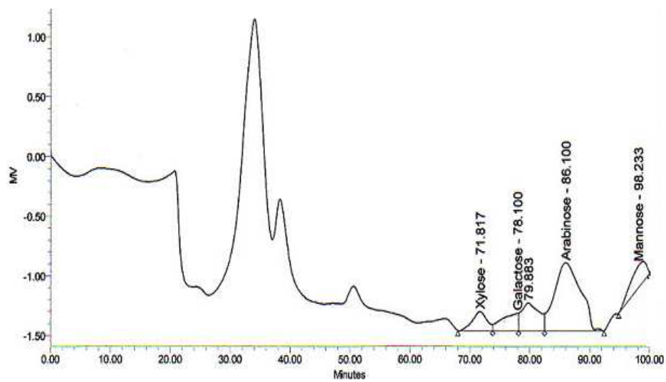
Figure 5. HPLC Chromatogram of Enzyme Hydrolysis Products Xyl : Xylose (RT = 71.817), Arabinose (86.1)
