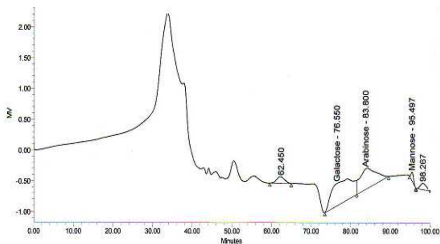
Figure 3. HPLC Chromatogram of Enzyme Hydrolysis Products Abfa : Arabinose (RT = 83.8)
