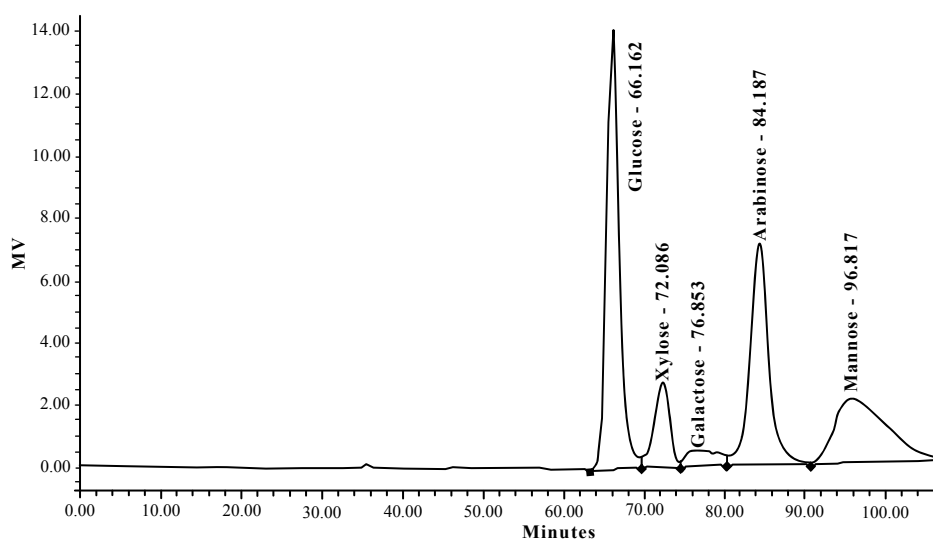
Figure 2. HPLC Chromatogram Standards : Xylose (RT = 72.086), Arabinose (RT 84.187)
