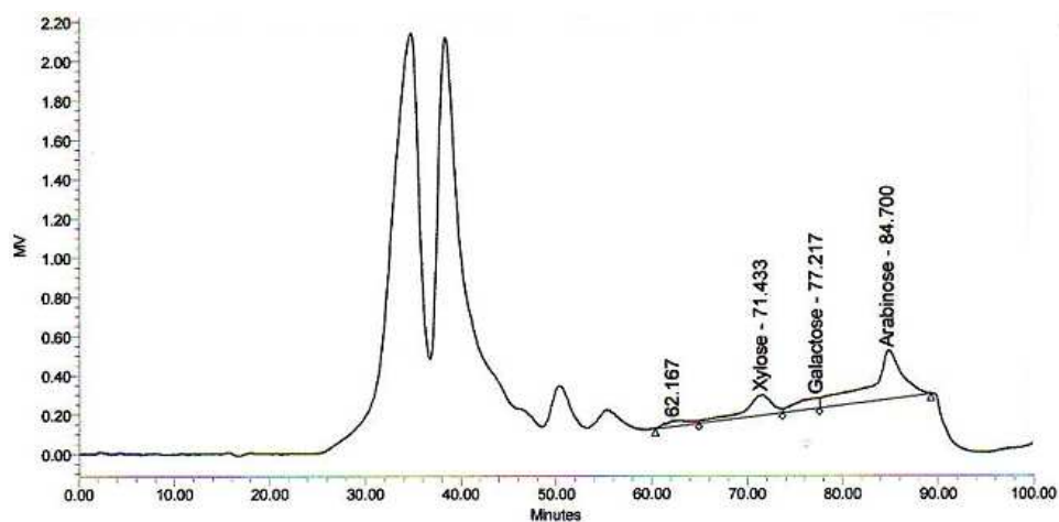
Figure 4. HPLC Chromatogram of Enzyme Hydrolysis Products Exo-xyl : Xylose (RT = 71.433), Arabinose (RT = 84.7)
