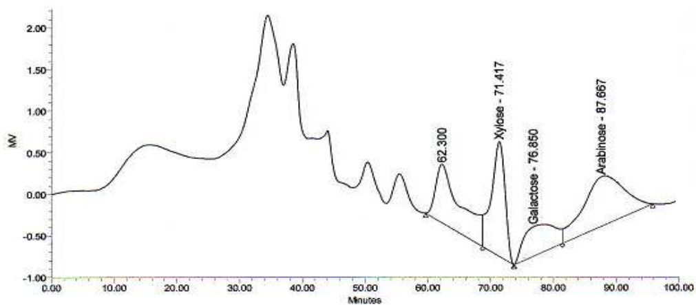
Figure 7. HPLC Chromatogram of Hydrolysis Products of Enzyme Mixture Abfa and Xyl : Xylose (RT = 71.417), Arabinose
