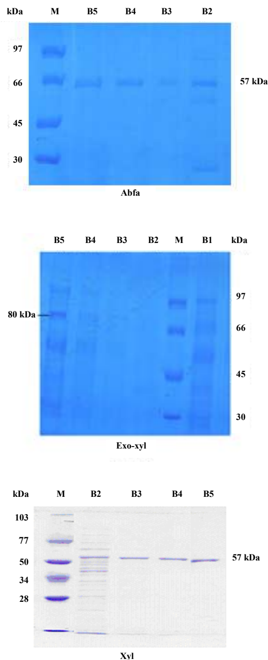
Figure 1. Electroforetogram of the Purified Enzyme by SDS-PAGE. \beta -xilosidase (Xyl), \alpha -L-arabinofuranosidase (Abfa), Exo-xylanase (Exo-Xyl) : M = Marker, B1 = Leaching into the Buffer B-1, B2 = Leaching into the Buffer B-2, B3 = Leaching into the Buffer B-3, B4 = Leaching into the Buffer B-4, B5 = Leaching into the Buffer B-5
