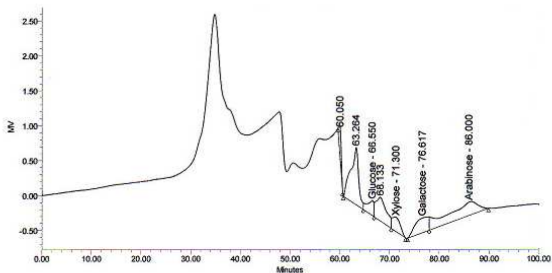
Figure 9. HPLC Chromatogram of Hydrolysis Products of Enzyme Mixture Abfa, Exo-xyl and Xyl : Xylose (RT = 71.3), Arabinose (RT = 86.0)
