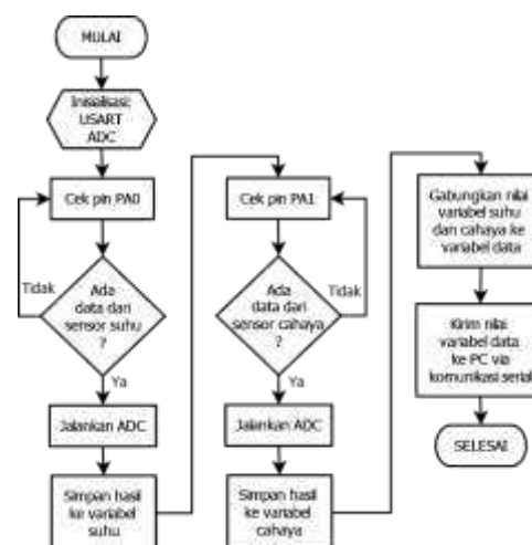
Gambar 8. Alur Program Mikropengendali
