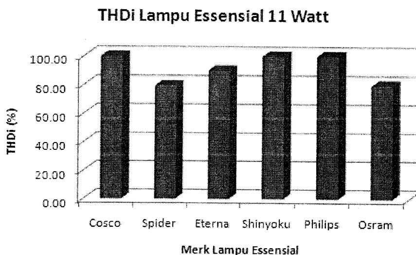
Gambar 8. Perbandingan THD i Lampu Essensial 11 Watt
