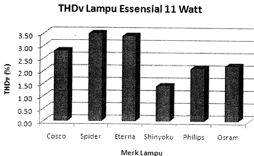
Gambar 7. Perbandingan THD v Lampu Essensial 11 Watt
