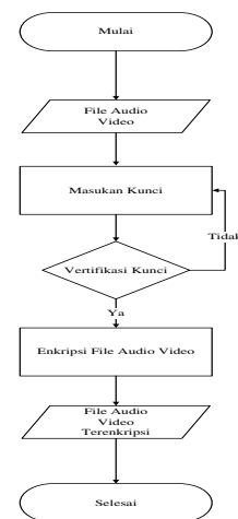
Gambar 2. Flowchart Enkripsi File Audio Video
