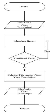
Gambar 3. Flowchart Dekripsi File Audio Video
