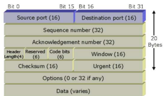
Gambar 4. Segmen TCP [7]
