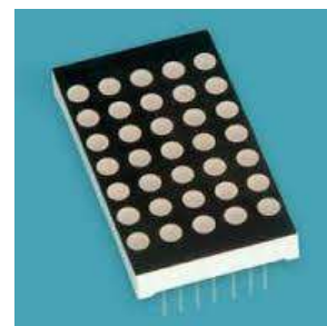
Gambar 3. Dot Matriks
