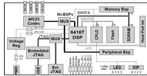
Gambar 1 Blok Diagram DSK TMS320C6416T
