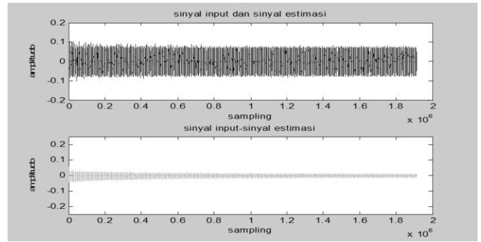
Gambar 9 Filter lengh 32 step size 0.005
