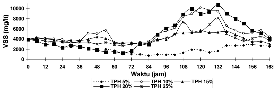
Figure 1. Consortium Growth Curve at pH 6,8 – 7,2; Temperature is at 28 °C
