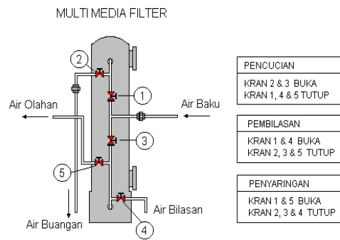
Gambar 3 : Diagram proses pengoperasian unit filter multi-media.
