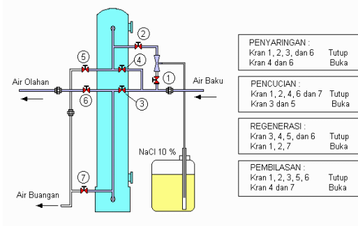
Gambar 6 : Skema pengoperasian filter penukar ion (softener).
