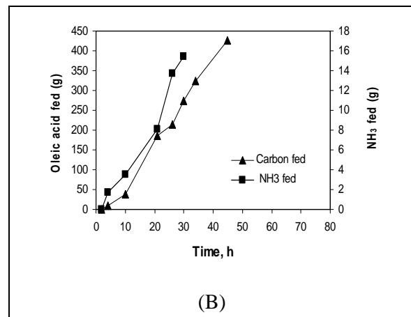
Figure 3. Time course of cell concentration, PHA content, and residual cell concentration (A); Amount of oleic acid and (NH 4 ) 2 SO 4 as NH 3 fed to the fermenter (B).
