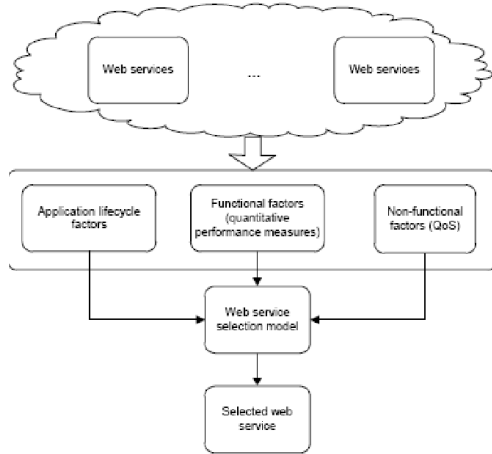
Figure 1 Generic Form of Web Service Selection Architecture
