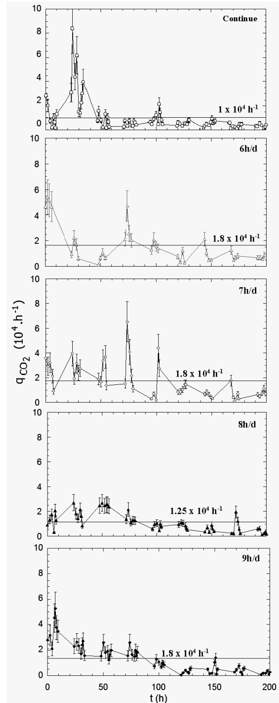
Figure 7. The Changes of q_{CO_2} at both of continuous illumination and photoperiodicity
