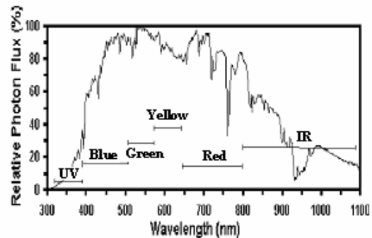
Figure 3. Earth surface sunlight spectrums composition in 12:00 noon [11].
