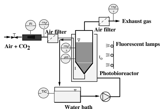
Figure 1. Experimental apparatus
