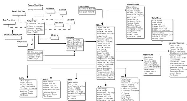
Gambar 7. ERD OLAP Entry.
