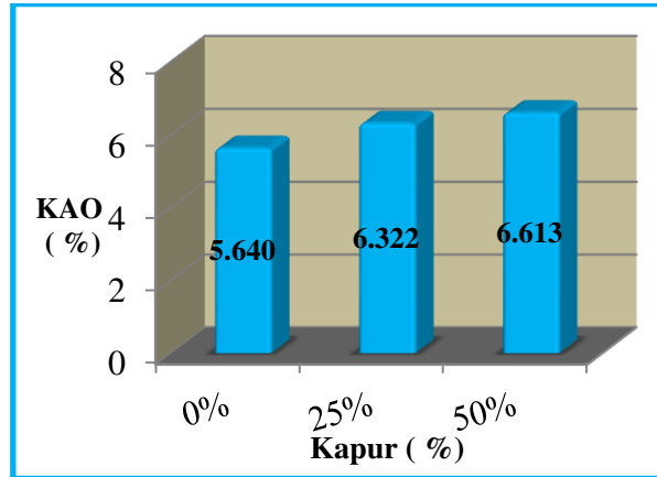
Gambar 7 Kadar Aspal Optimum Masing-masing Campuran
