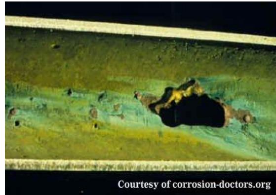
Gambar.4. Lobang karena Erosion Corrosion
