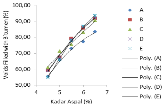
Gambar 8. Kadar aspal vs VFB
