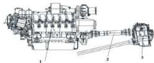
Gambar 5.2. Perencanaan V-Drive gearbox
