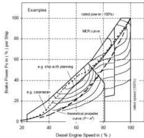
Grafik 5.1 Kurva engine propeller matching
