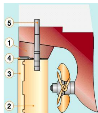
Gambar.1. Rudder Conventional.
