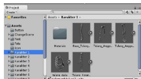
Gambar 10 Export Objek
