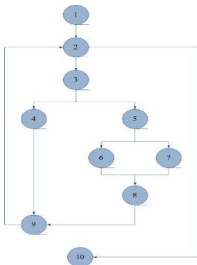
Gambar 16. Flowgraph SwipeObject
