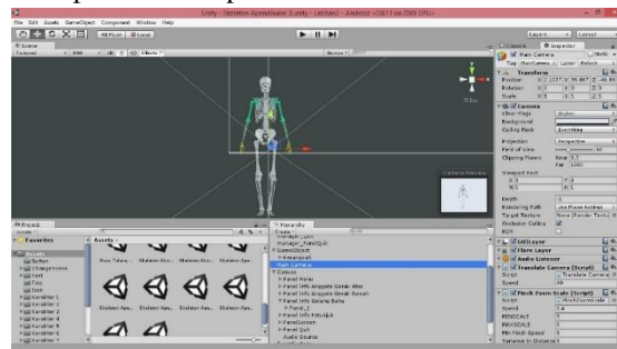
Gambar 12 Camera Preview
