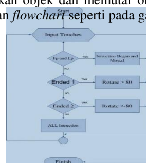
Gambar 15. Flowchart SwipeObject
