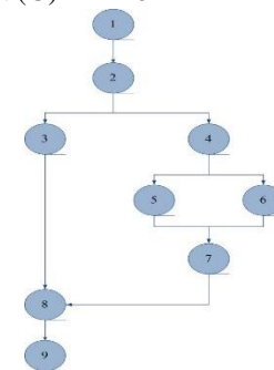
Gambar 18 Flowgraph PinchZoom
