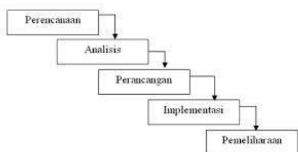
Gambar 1 Waterfall
