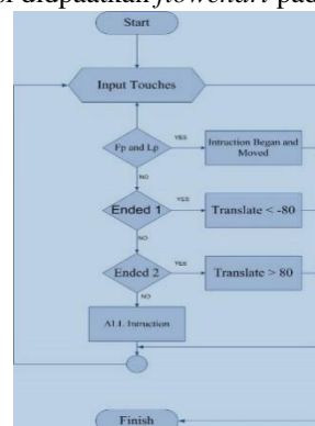
Gambar 19 Flowchart ShiftObject
