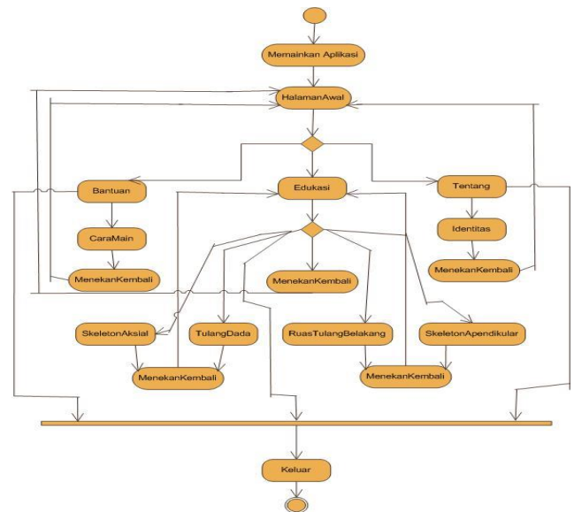
Gambar 7 Diagram Activity
