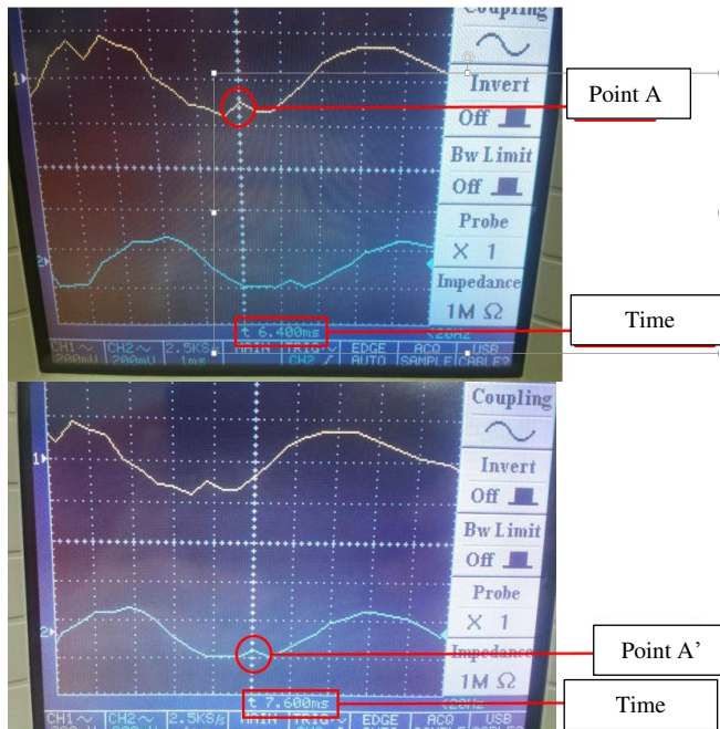
Picture 5 Comparison of Two Delayed Signal over Time
