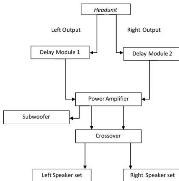
Picture 3 Delay Module Installation Diagram
