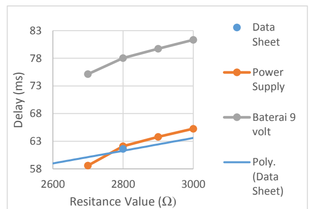
Picture 4 The Chart of Delay Data Comparison
