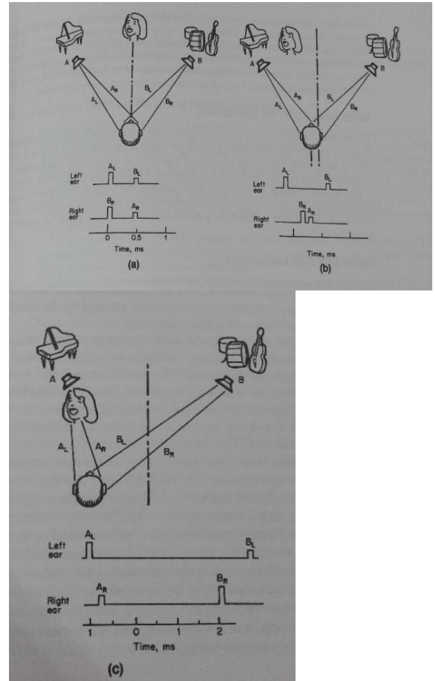
Picture 7 Illustration by Benson & Whitaker a) centered listening b) a bit left listening c) near the left speaker listening
