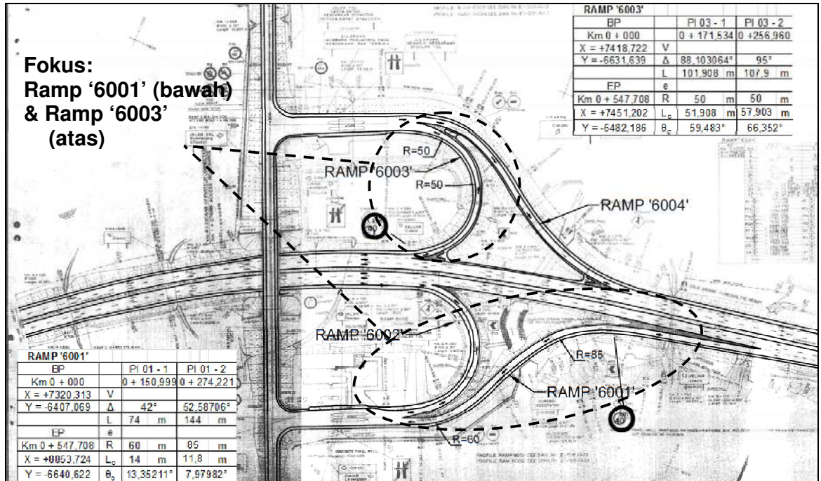
Gambar 3 Denah Simpang Susun Baros
