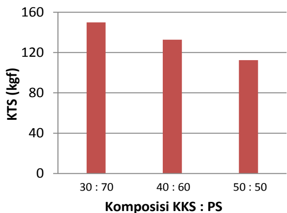
Gammar 4. Kuat Tarik Sekrup (KTS) Block Board
