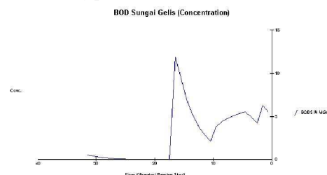
Gambar 2. Grafik Hasil Running Program QUAL2E
