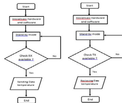
Gambar 7 Flowchart sistem
