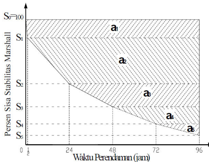
Gambar 1. Gambaran skema kurva keawetan(Crauss at al. , 1981)
