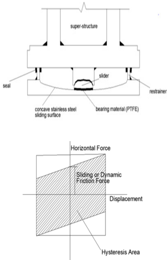
Sumber : Modelling Aspects of Structures Isolated With The Frictional Pendulum System (Jose, et.al., 1998)
