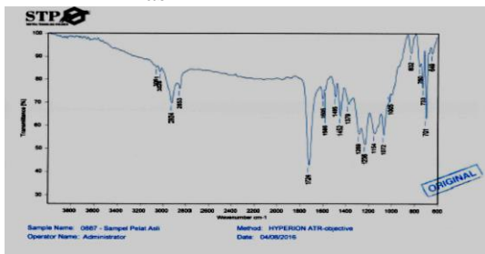
Lampiran 1. Spektrum FTIR sampel pelat asli
