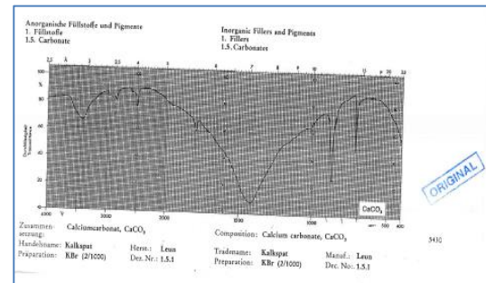
Lampiran 4. Spektrum FTIR referensi hummel No. 5430
