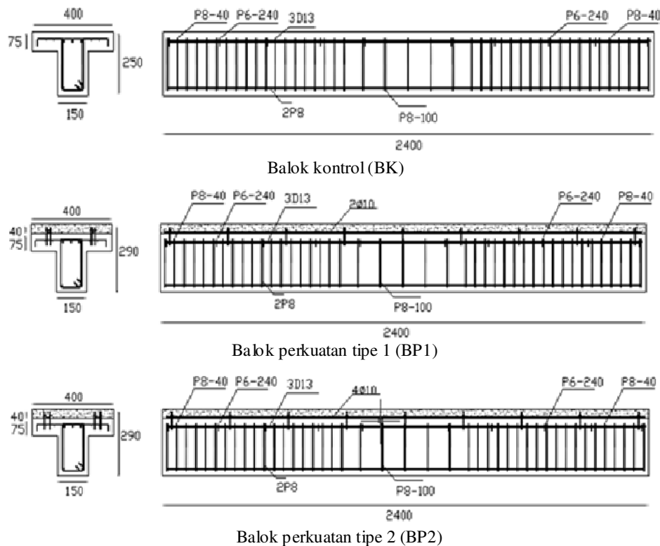
Gambar 3. Penampang model benda uji (Haryanto, 2011)
