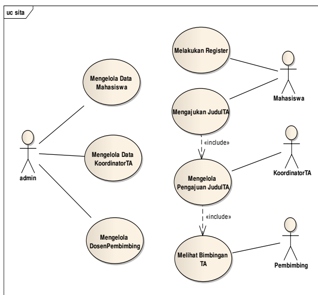
Gambar 2. Use Case Diagram SITA
