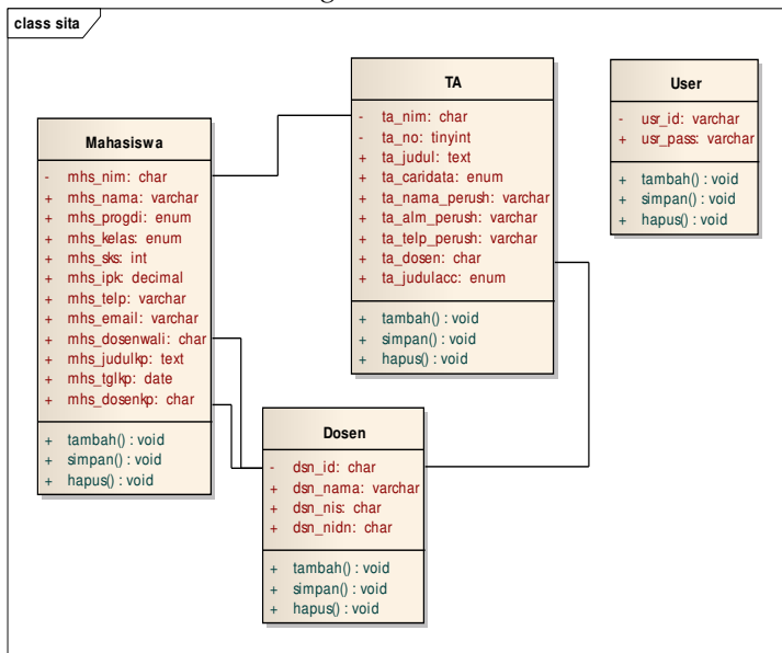
Gambar 7. Class Diagram SITA
