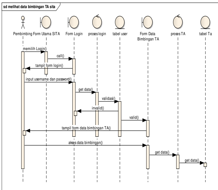
Gambar 6. Sequence Diagram Melihat Data Bimbingan TA
