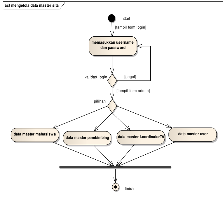
Gambar 4. Activity Diagram Admin Mengelola Data Master SITA
