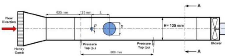
Gambar 1. Instalasi penelitian
