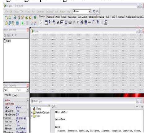
Gambar. 3. Tampilan Delphi
