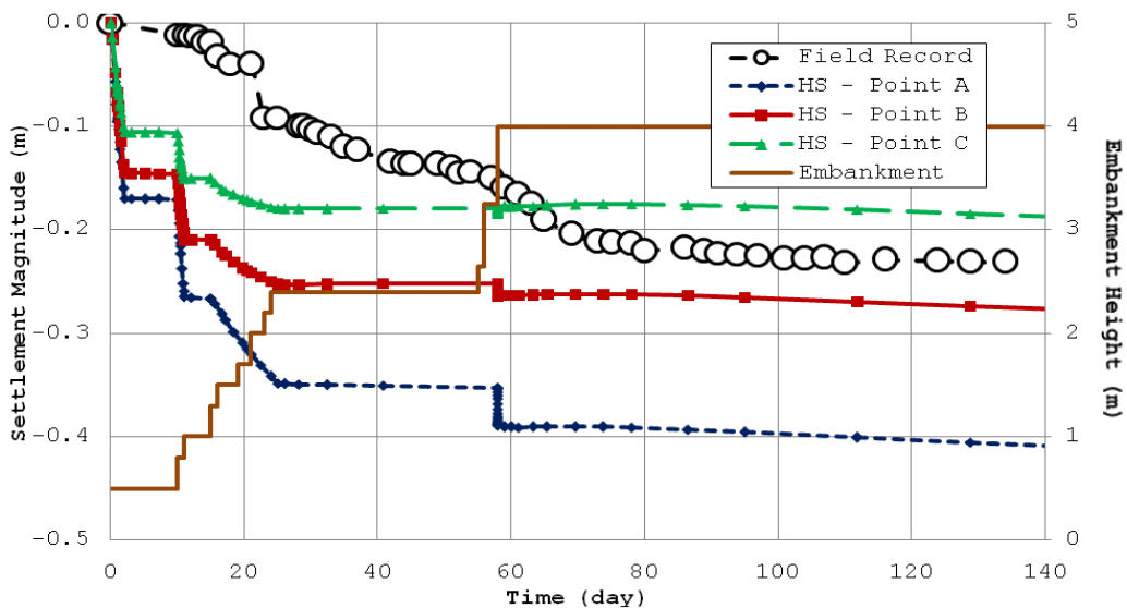
Figure 18. Settlement behavior of foundation soils at toes of the embankment: (a) MC model and (b) HS model
