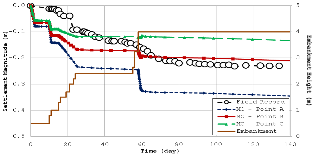
Figure 17. Settlement behavior of foundation soils at the center of the embankment
