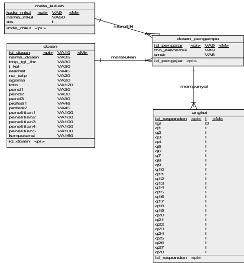
Gambar 4 Physical Data Model
