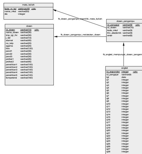
Gambar 3 Conceptual Data Model
