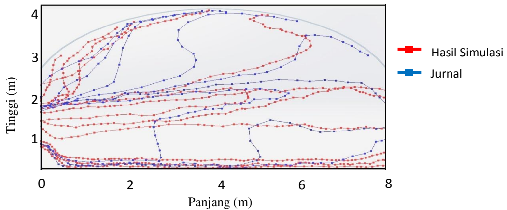
Gambar 6. Perbandingan garis Isoline Teperatur sample house hasil simulasi dengan greenhouse pada Jurnal Catherine Baxevanou ( Numerical simulation of solar radiation, air flow and temperature distribution in a naturally ventilated tunnel greenhouse , 2009)
