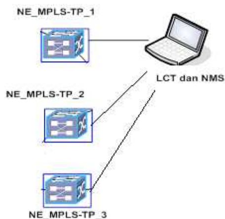
Gambar 6. Desain Topologi Point-to-Point
