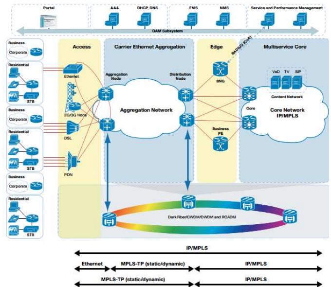
Gambar 1. Ilustrasi Pengimplementasian MPLS-TP [1]
