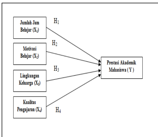
Gambar 1 Model Penelitian
