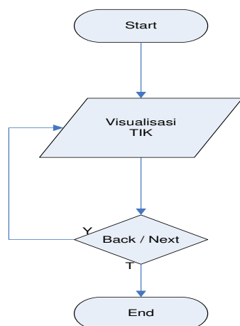
Gambar 1 Flowchart TIK
