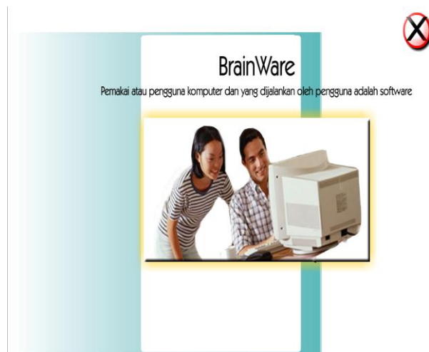
Gambar 13 Interface Brainware
