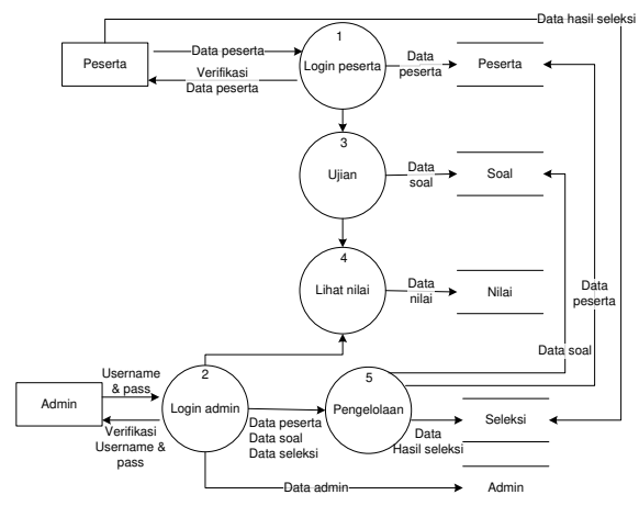
Gambar 3.3 DFD Level 1
