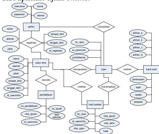
Gambar 3.9 Entity Relationship Diagram
