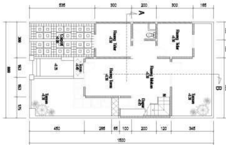
(a). denah lantai 1
