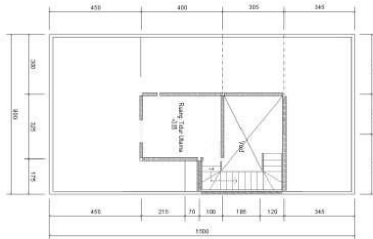
(b). denah lantai 2
