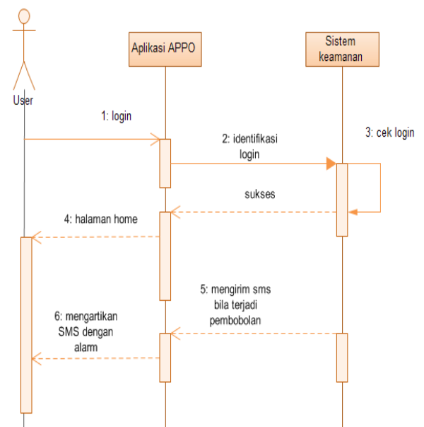
Gambar 10. Sequence diagram fitur alarm
