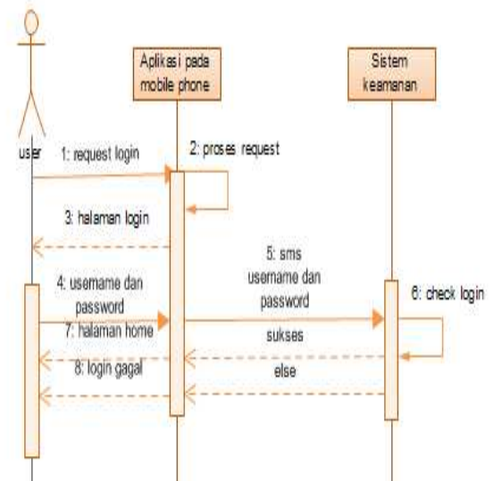
Gambar 5. Sequence diagram fitur login
