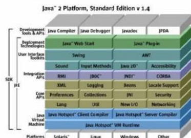
Gambar 1. Java 2 Platform Standar Edition
