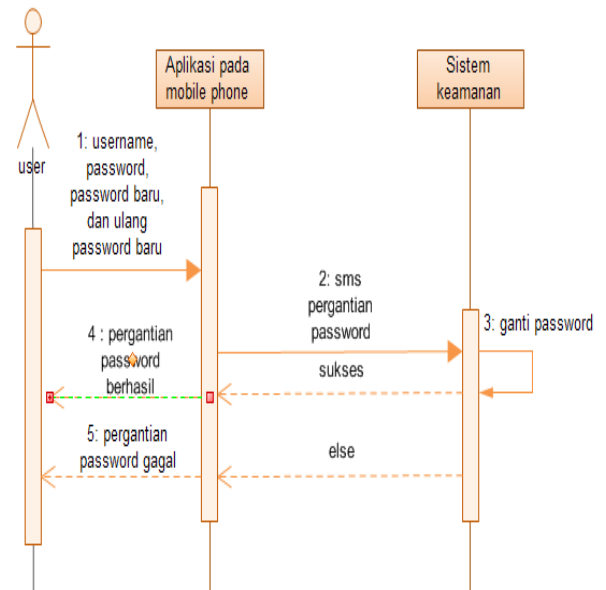
Gambar 9. Sequence diagram fitur ganti password
