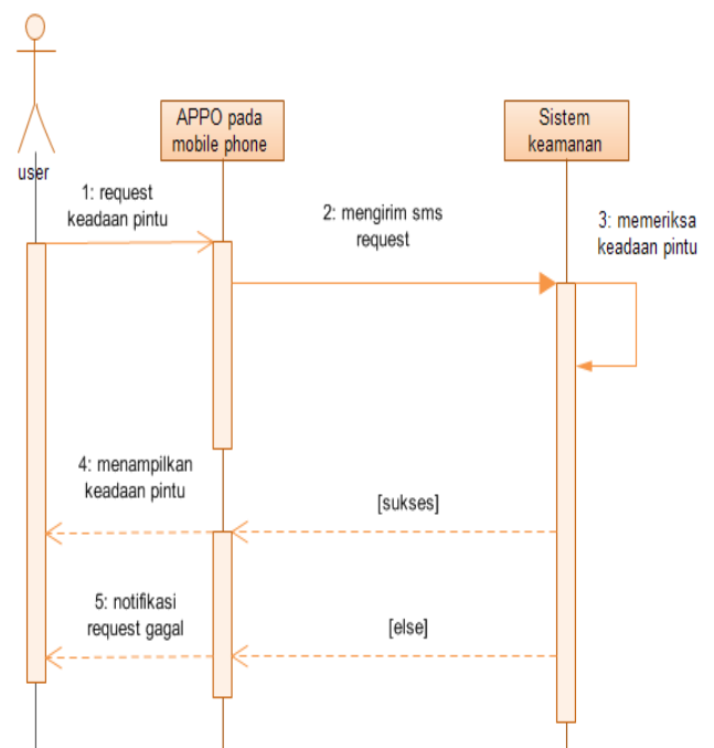
Gambar 6. Sequence diagram fitur request keadaan pintu
