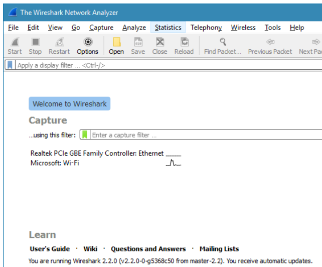
Gambar 11. Wireshark
