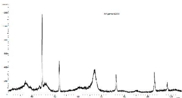
Gambar 2. hasil analisa XRD katalis Ni/ \gamma\text{Al}_2\text{O}_3
